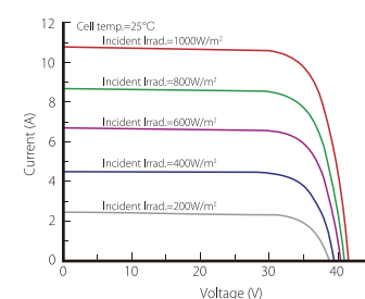
Current-Voltage Curve (LR4-60HPH-360M)
